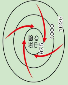
南半球氣旋
